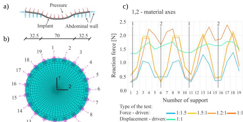
Fig. 1. a) Cross-section of the numerical model; b) Numerical model; c) Reaction forces in supports
