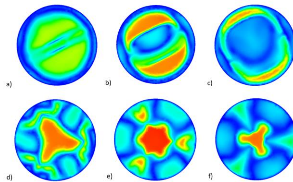
Fig. 2. Flow characteristics for the opening angle of the two-disc valve: a) 0°, b) 20°, c) 40°, for three-leaflet valve: d) 0°, e) 20°, f) 40°
