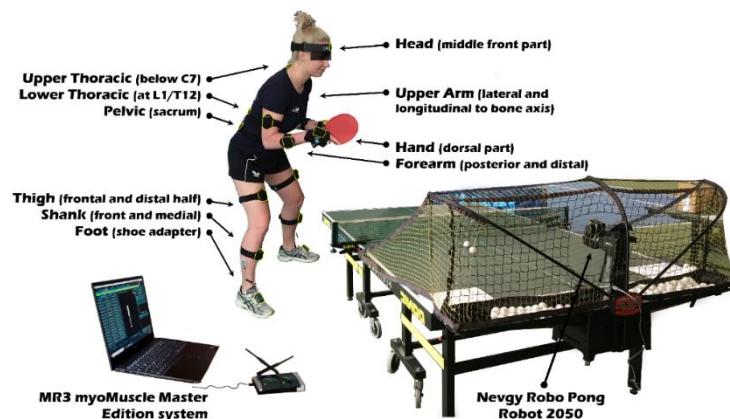
Fig. 1. Measurement site and scheme.
