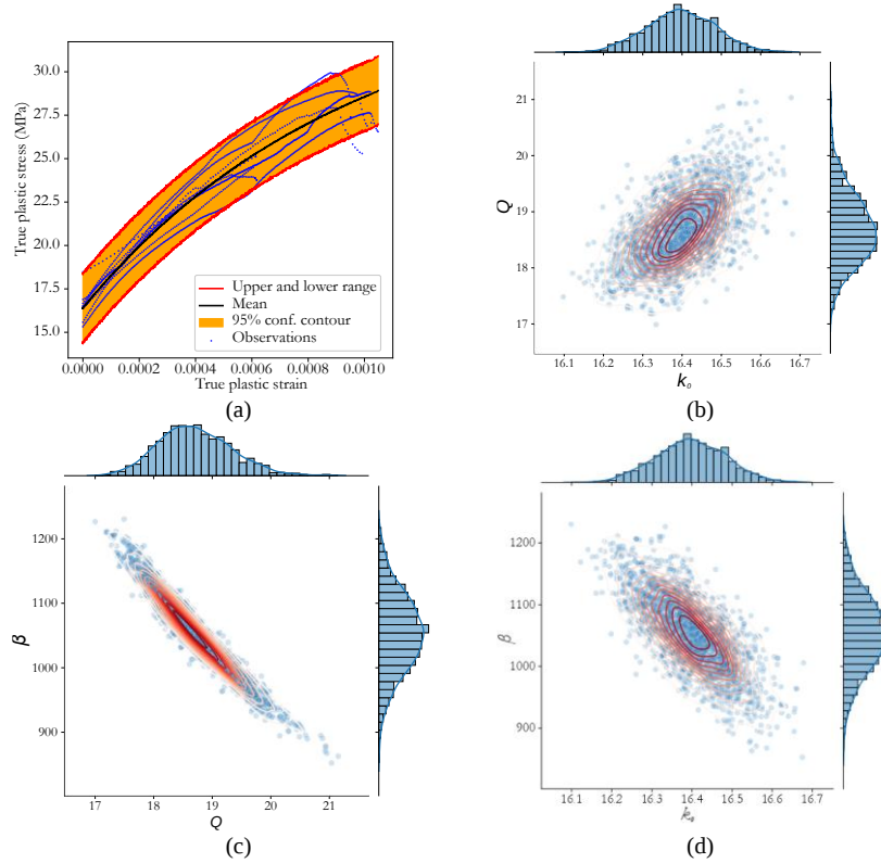
Fig. 2. Model prediction. (a) Predicted true stress-strain curves and their uncertainty bands with 95% confidence contour, (b-d) Joint probability plots of the model pair wise parameters ( k_0 and Q are in MPa while \beta is unitless)
